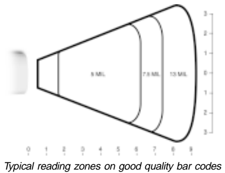
Typical reading zones on good quality bar codes
